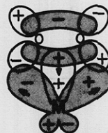
Figure 3. Bonding orbitals for class I dioxygen complexes.
